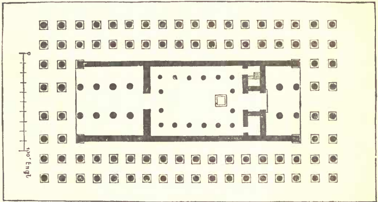
GROUND-PLAN OF DOUBLE PERIPTERAL
